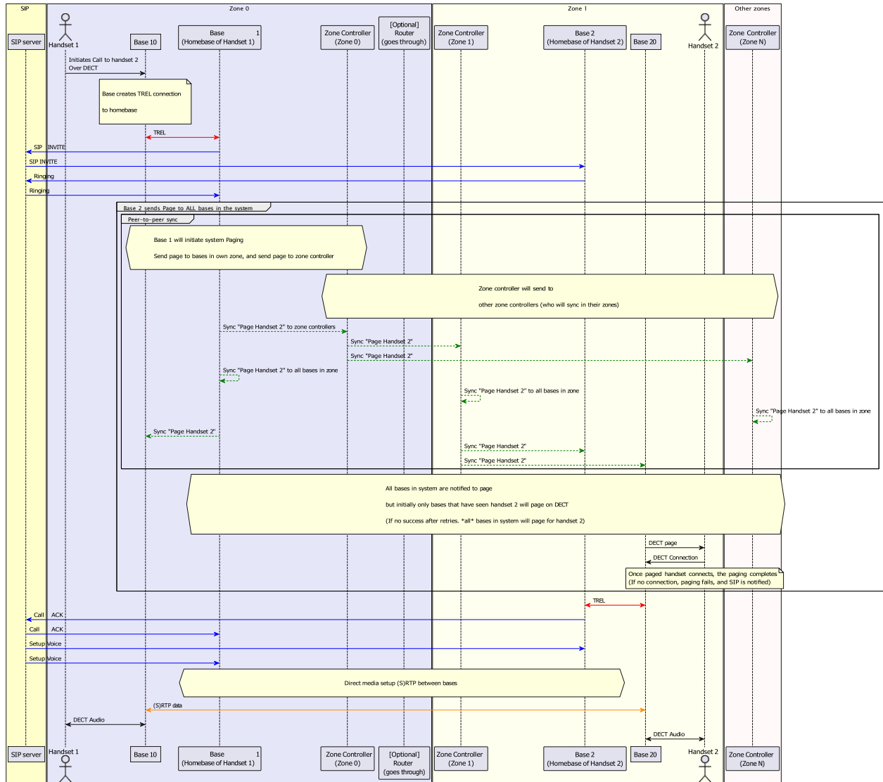
Figure 19: Call not in home base
