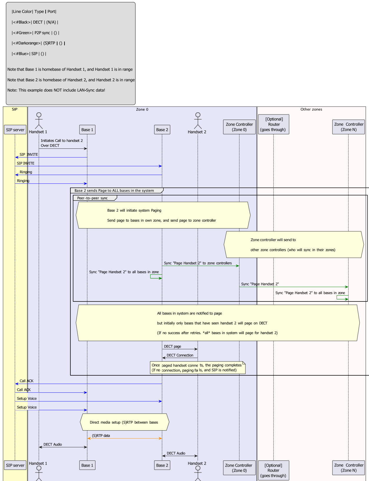
Figure 18: Multi-zone calls inside zone
